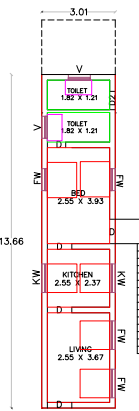
PLAN - GROUND FL ( PROPOSED )
