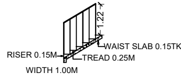
STAIRCASE DETAILS
