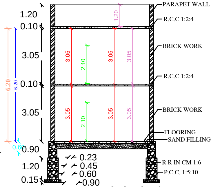
SECTION AB
