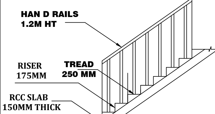
STAIRCASE DETAILS SCALE 1:50
