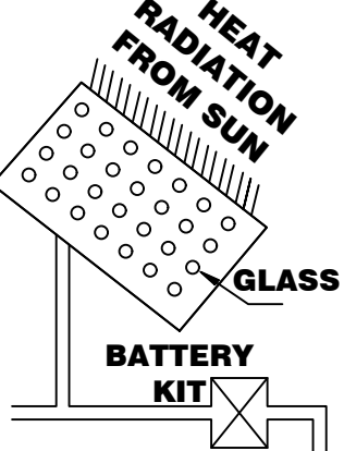
SOLAR SYSTEM
