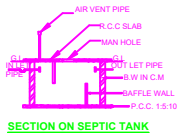
SECTION ON SEPTIC TANK
