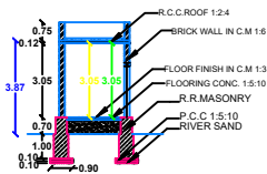
SECTION ON A - B
