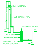
RAIN WATER HARVESTING SYSTEM
