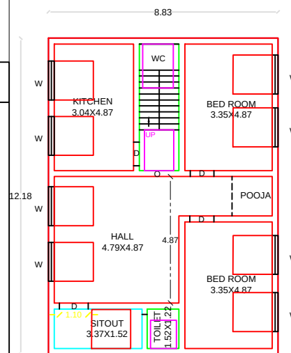
PRO GF PLAN
