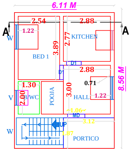
PLAN - GROUND FLOOR
