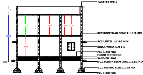
SECTION AB
