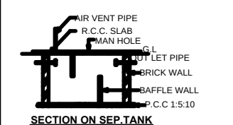
SECTION ON SEPT.TANK
