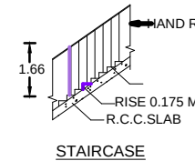
STAIRCASE
