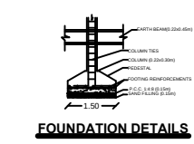
FOUNDATION DETAILS
