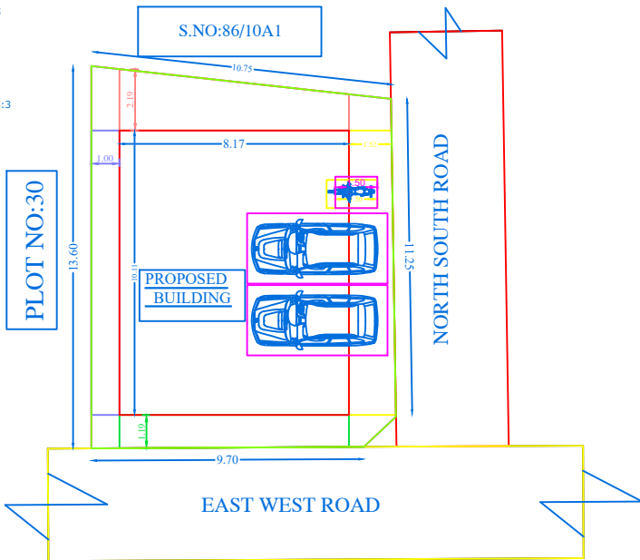
SITE PLAN
