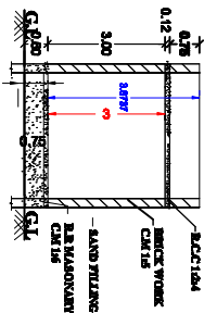
SECTION ON "BB"
