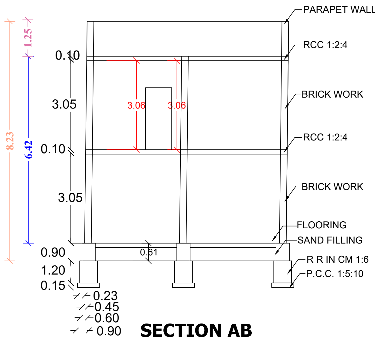
SECTION AB
