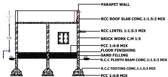
SECTION AB
