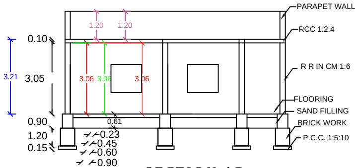
SECTION AB
