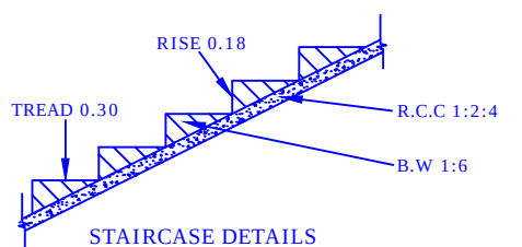
STAIRCASE DETAILS
