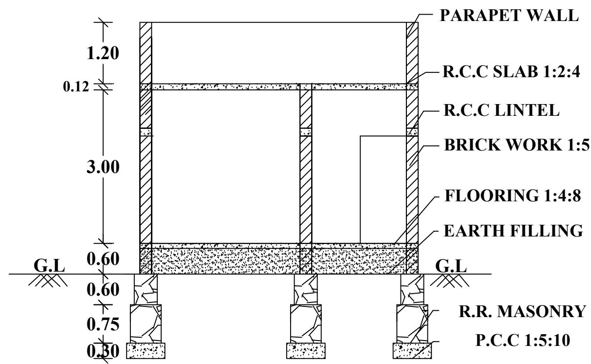
"SECTION "AB"
