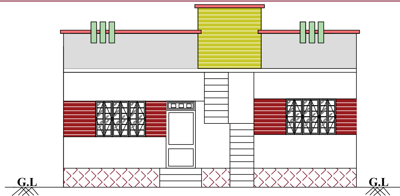
FRONT ELEVATION
