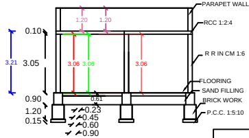
SECTION AB
