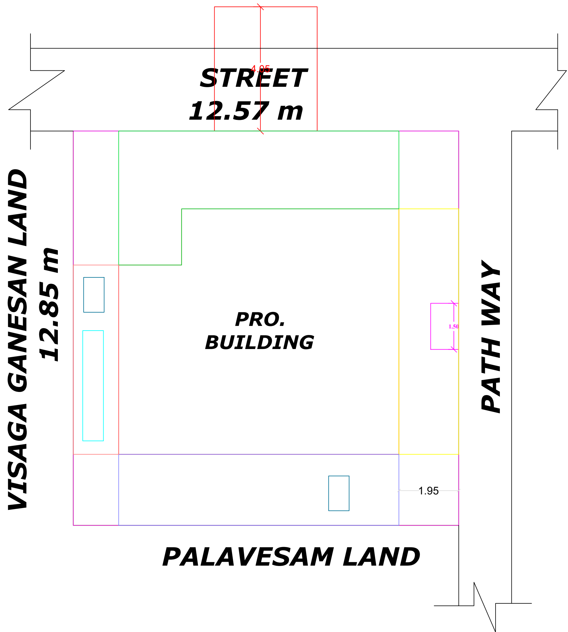
SITE PLAN
