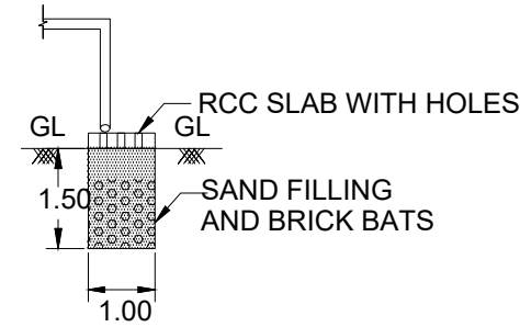
SECTION OF BS
