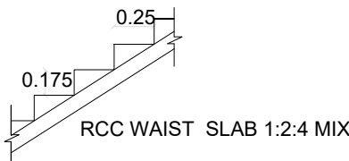
STAIRCASE DETAILS
