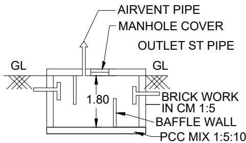
SECTION ON SEPTICTANK
