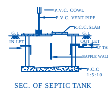
SEC. OF SEPTIC TANK
