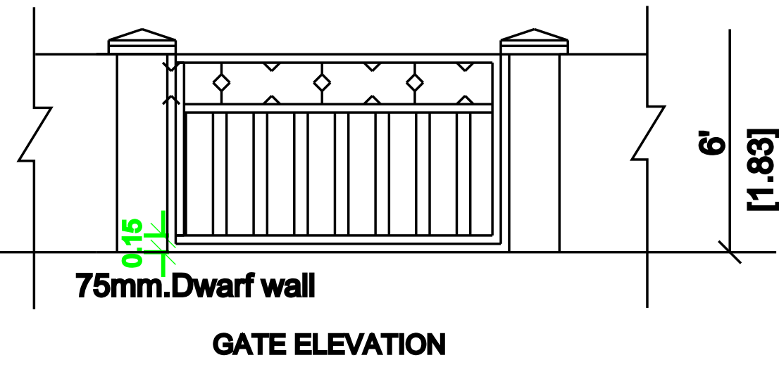
GATE ELEVATION
