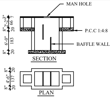
SEPTIC-TANK DETAIL
