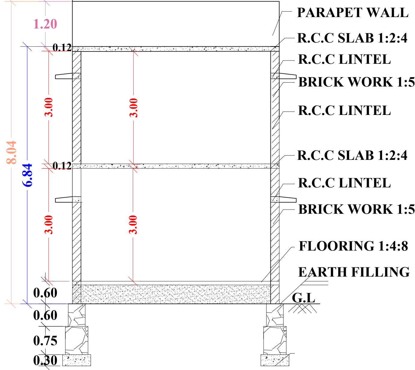
"SECTION "AB"
