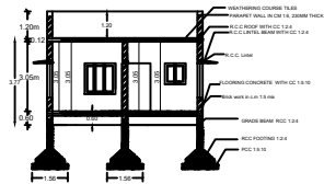
SECTION NON-AA
