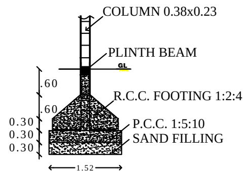
COLUMN DETAILS
