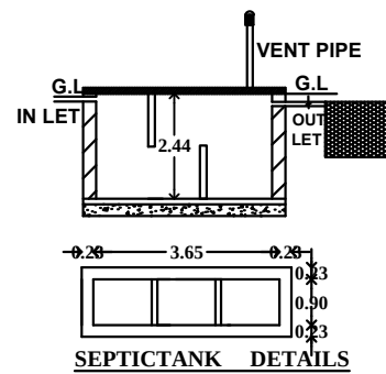
SEPTICTANK DETAILS
