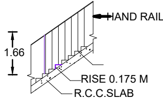
STAIRCASE
