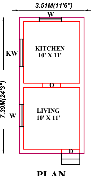
PLAN
