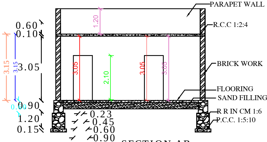
SECTION AB
