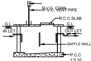
SEC. OF SEPTIC TANK
