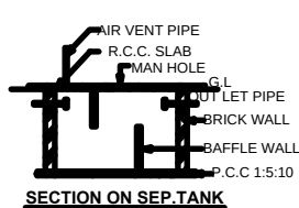
SECTION ON SEP.TANK
