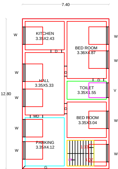
PROPOSED GF PLAN
