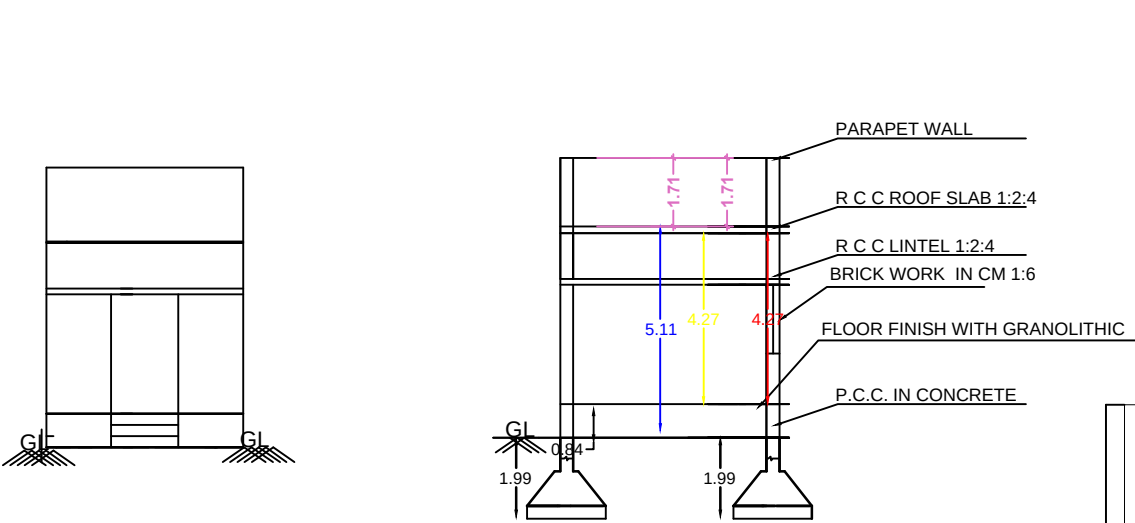
ELEVATION SECTION ON AA
