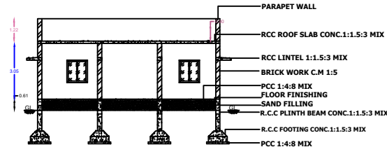
SECTION AB
