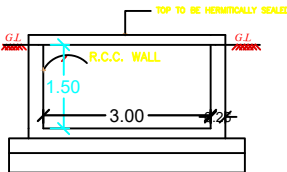
RWH SECTION
