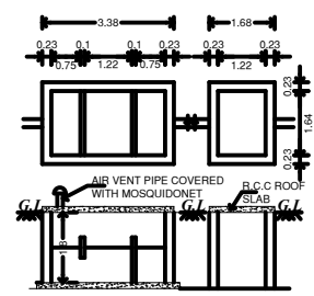
PLAN&SECTION OF SEPTIC TANK 'U' TRAP PROVIDED
