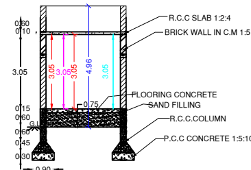
SECTION AB
