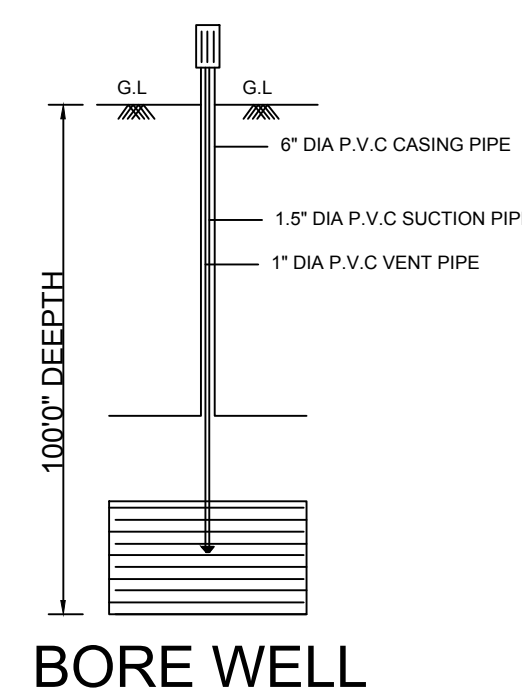
BORE WELL
