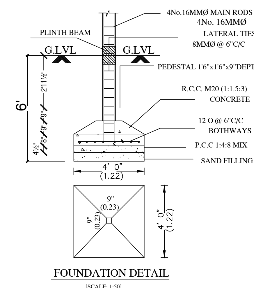
FOUNDATION DETAIL
