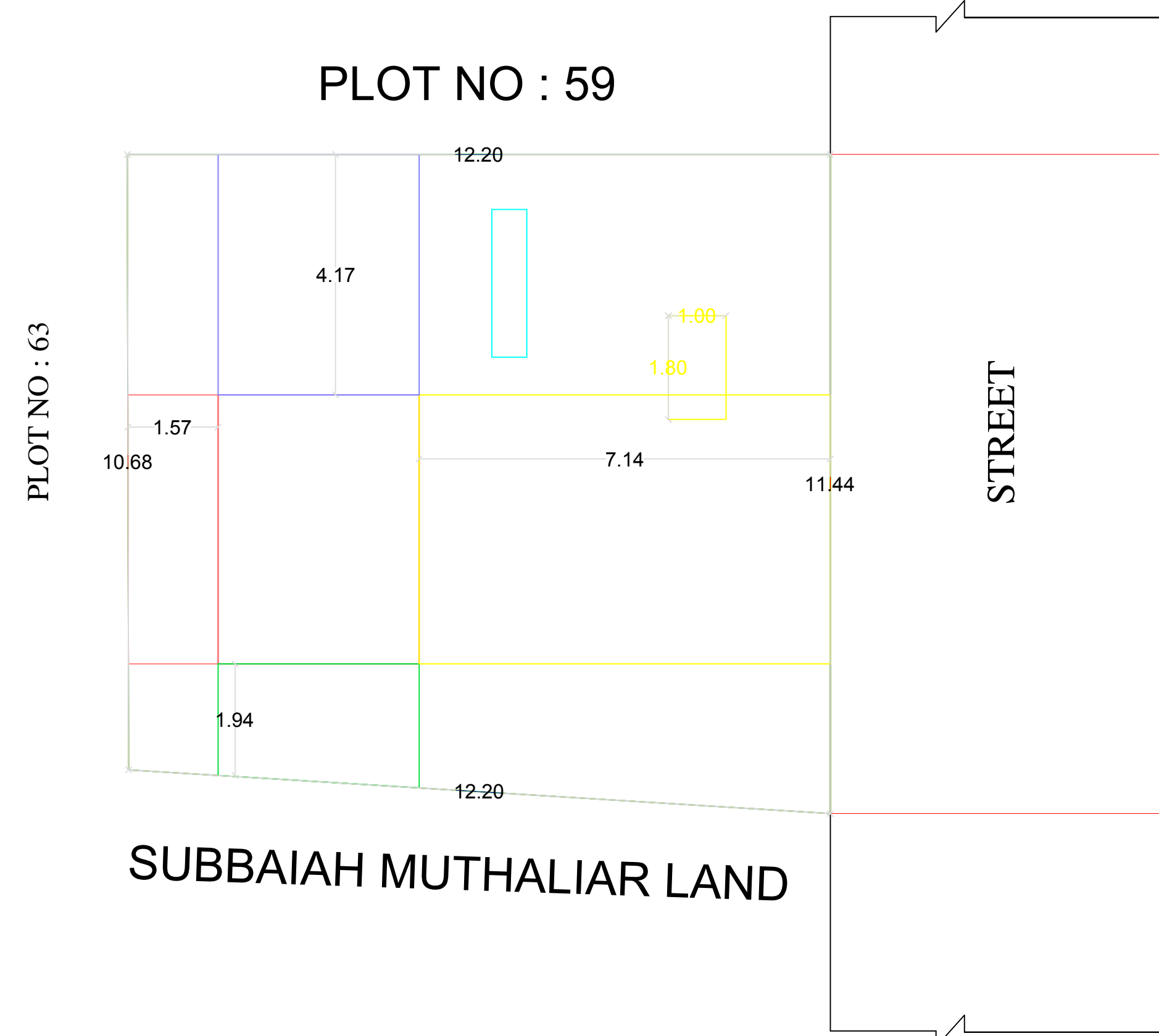
SITE PLAN
