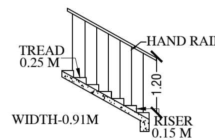
WIDTH-0.91M
