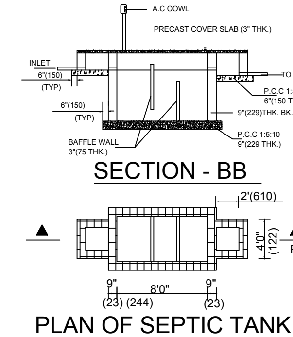
PLAN OF SEPTIC TANK
