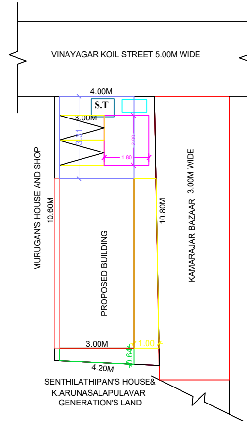
SITE PLAN
