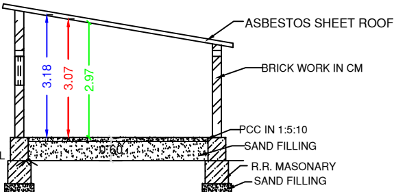
SECTION "AB"
