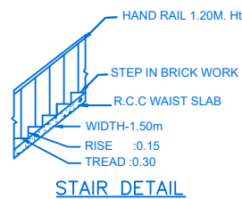
STAIR DETAIL
