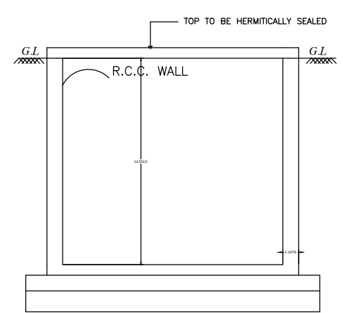
RWH_CAPACITY_L=5000LTRS
