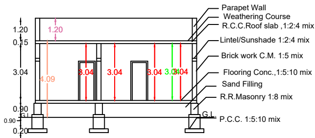
SECTION on R-K
