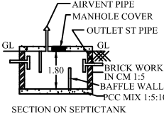
SECTION ON SEPTICTANK
