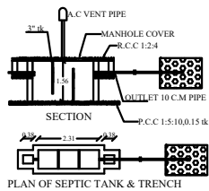
PLAN OF SEPTIC TANK & TRENCH
