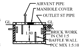
SECTION ON SEPTICTANK
