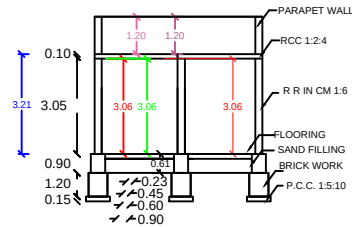
SECTION AB
