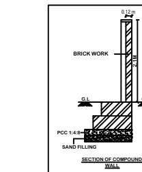
SECTION AB
