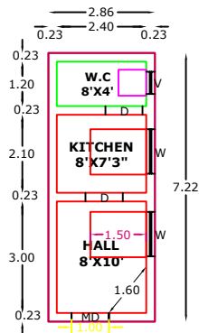
GROUND FLOOR RESIDENTIAL PLAN
