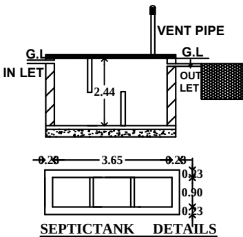
SEPTICTANK DETAILS
