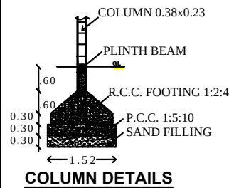
COLUMN DETAILS
