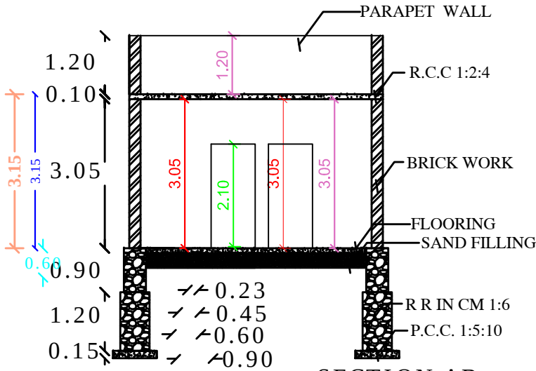
SECTION AB
