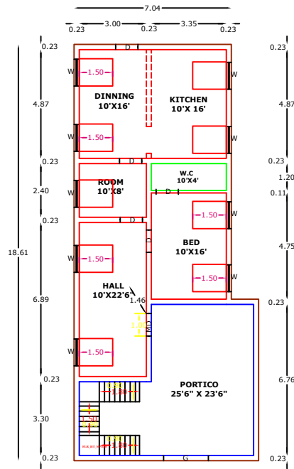
EXT GROUND FLOOR RESIDENTIAL PLAN
