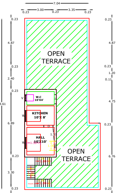
PRO FIRST FLOOR RESIDENTIAL PLAN
