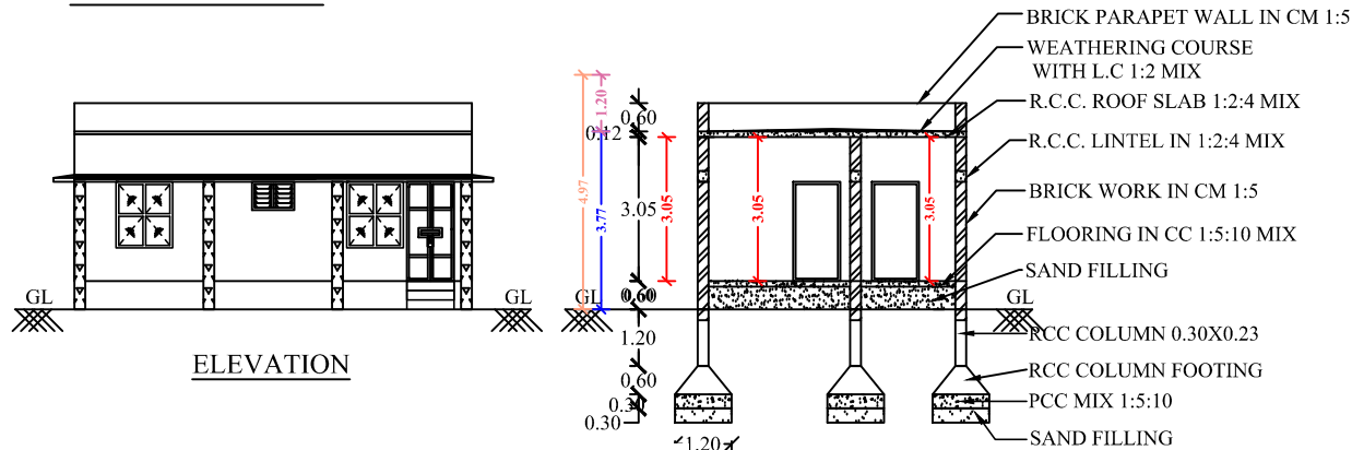
SECTION OF "AB"
